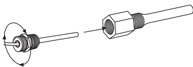
Thermowell placement in pipe
